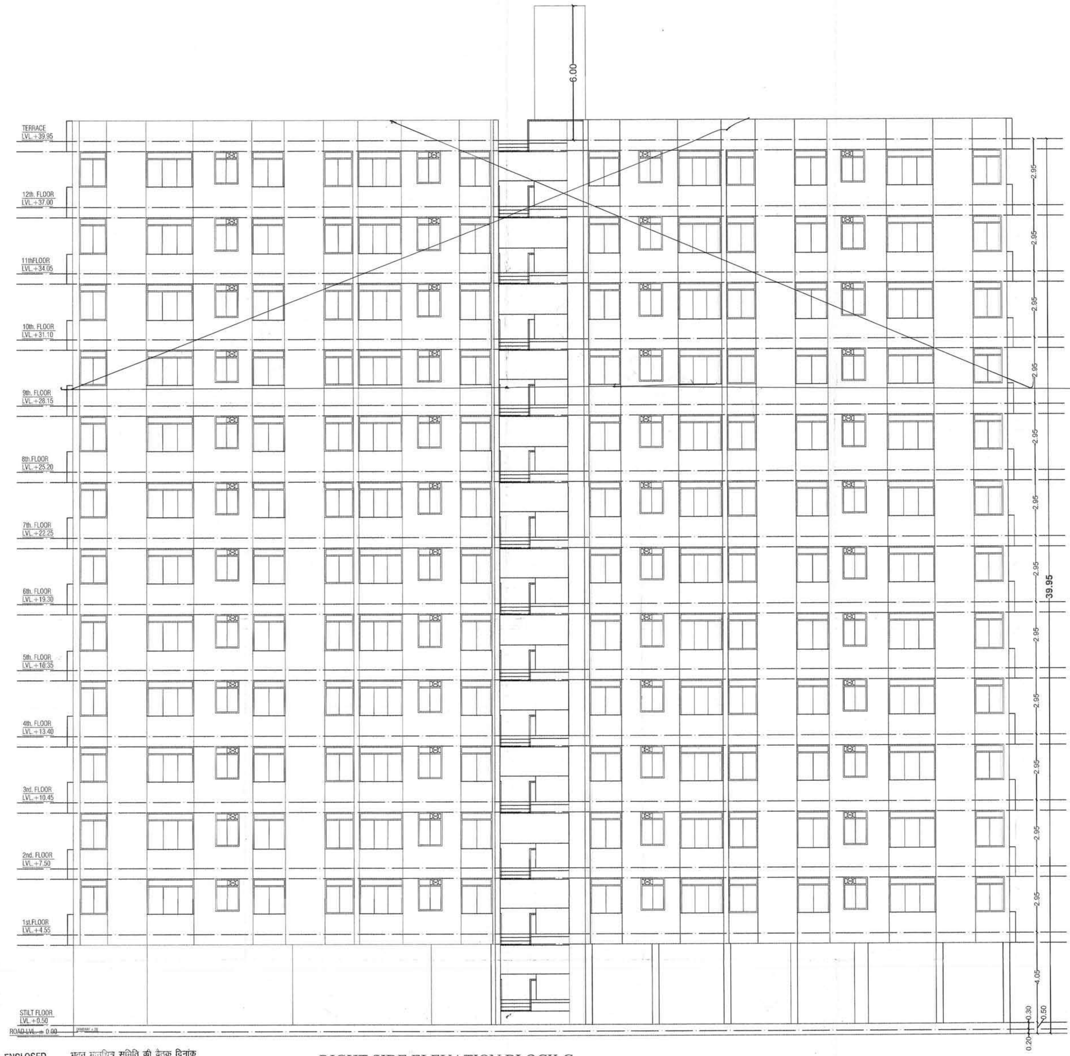
RIGHT SIDE ELEVATION BLOCK C
