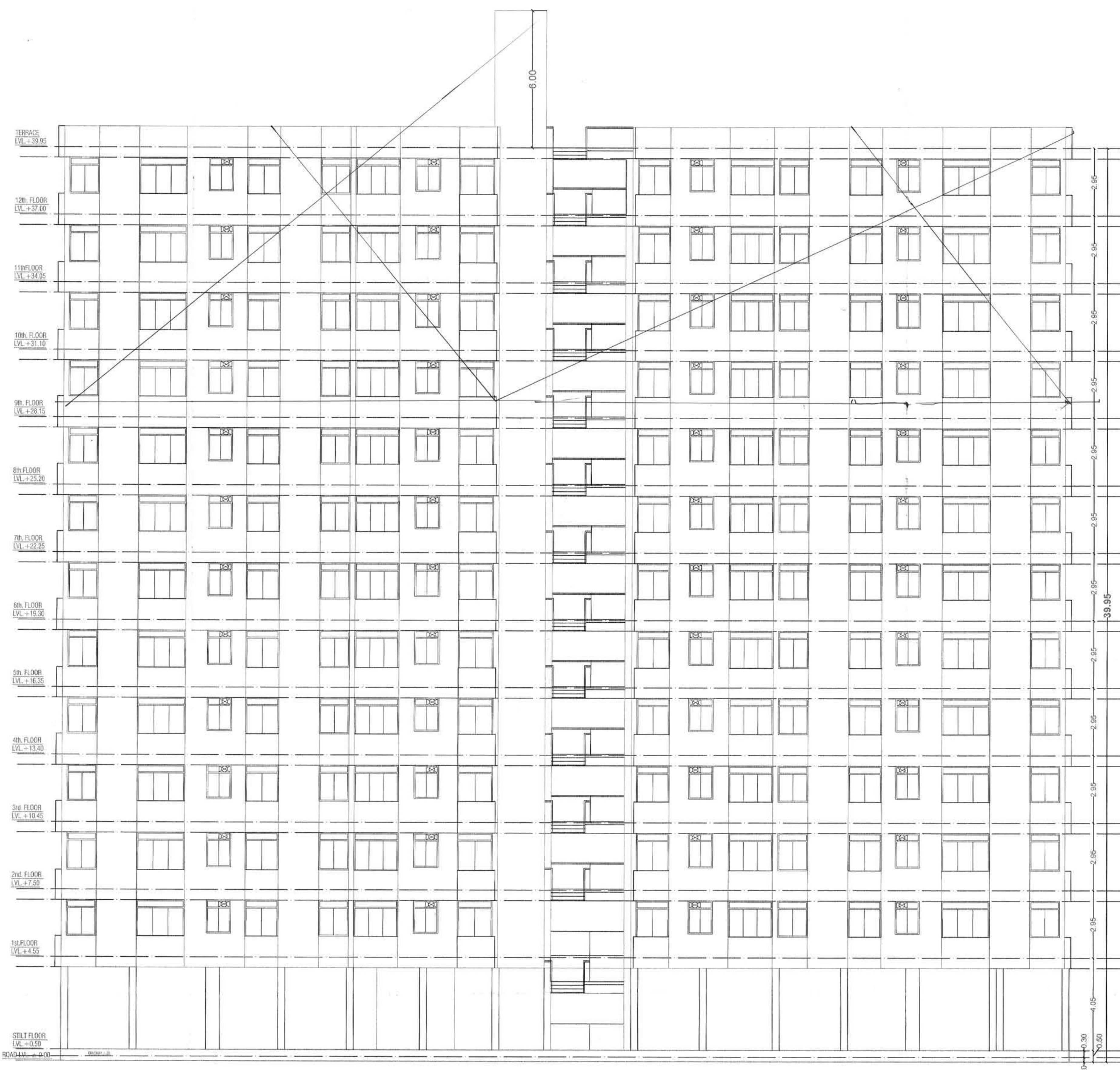
RIGHT SIDE ELEVATION BLOCK D
